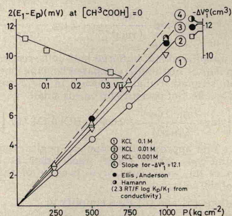
Fig. 4. 2(E_1 - E_p) = 2.3 RT/F \log k'_p/k'_1 = f(p) at zero acetic acid concentration, in 0.1, 0.01, and 0.001M KCl. Inserts: extrapolation of 2(E_1 - E_p) to zero KCl concentration and corresponding -\Delta V_1^\circ value ( 11.6 \text{ cm}^3 \text{ mole}^{-1} ). 2.3 RT/F \log K_p/K_1 and \Delta V_1^\circ from conductivity data [Ellis and Anderson (8); Hamann (9, 10)] are indicated together with the limiting slope of 2(E_1 - E_p) = f(p) for -\Delta V_1^\circ = 12.1 .
