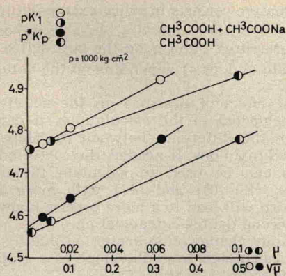
Fig. 3. Extrapolation of pK' and pK'_p values obtained at zero acetic acid and acetate buffer concentration, to zero KCl concentration; \mu scale, acetic acid; \sqrt{\mu} scale, acetate buffer. p^*K'_p at 1000 kg \text{cm}^{-2} is calculated from the slope of (E_1 - E_p) = f(p) at 1 atm for acetic acid; p^*K'_p = pK'_{1000} for acetate buffer where (E_1 - E_p) = f(p) is linear.
